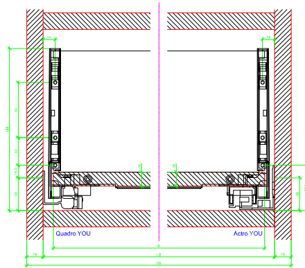
AVT YDU with Steel Rear Panel
