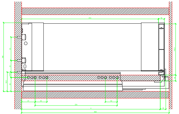
AVT YOU with Aluminium Profile
