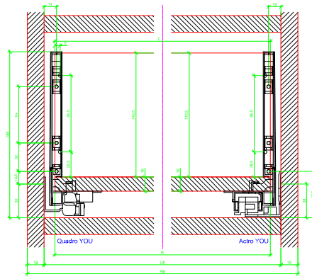
AVT YDU with Wooden Panel
