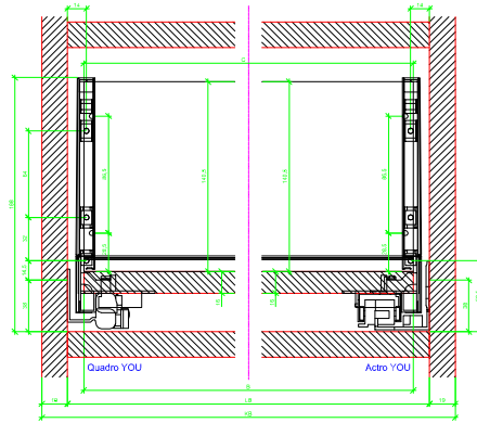
AVT YDU with Aluminum Profile
